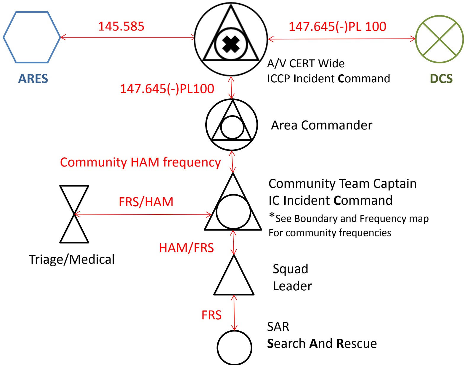
CERT Radio communication flow
